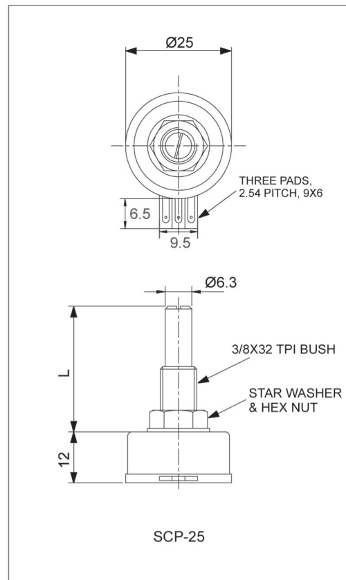
Dimensional Diagram
