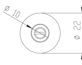
Dimensional Diagram
