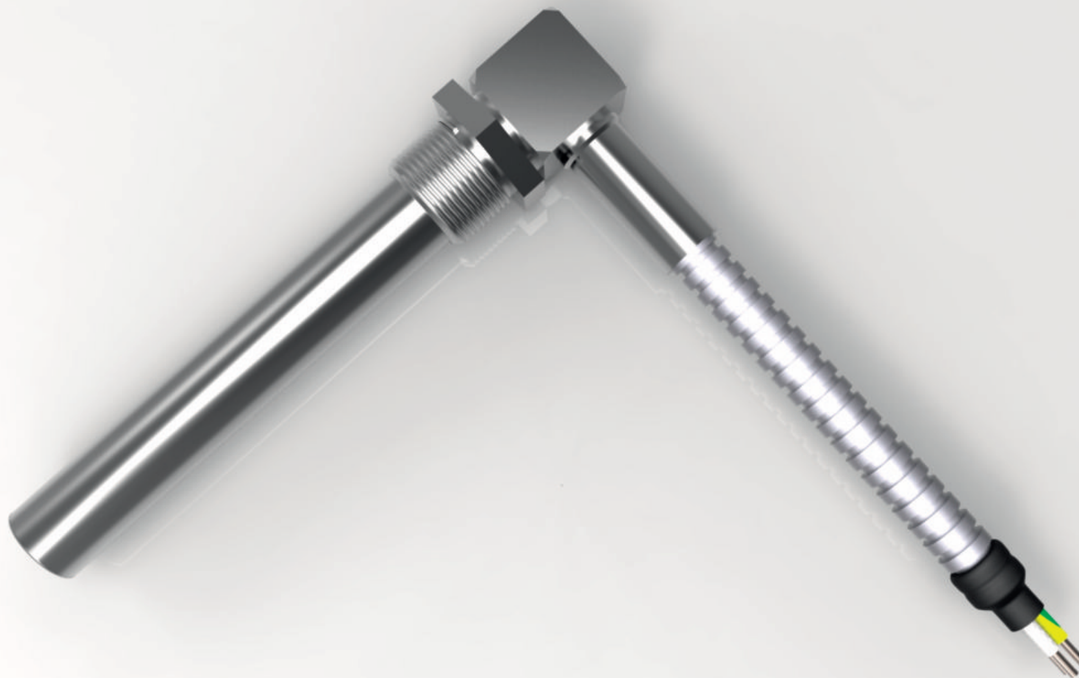
28a CARTRIDGE HEATER Special design, cables protected by flexible corrugated tube
