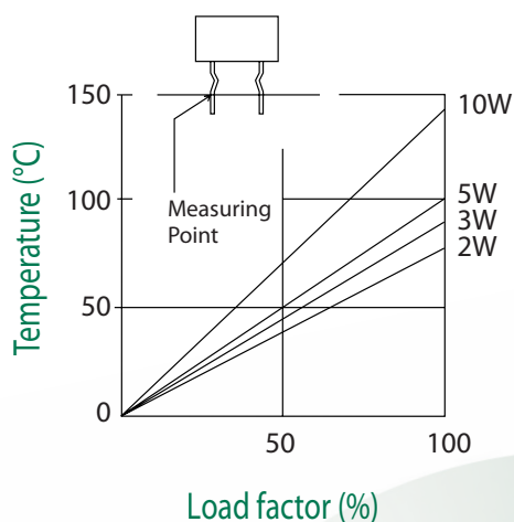
TEMPERATURE RISE CHART
