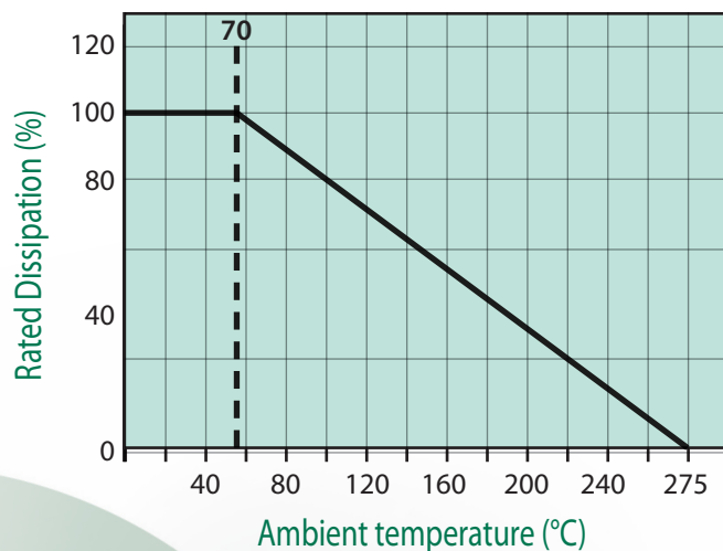
DERATING CURVE
